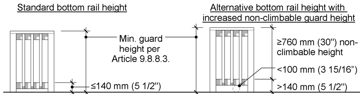
Figure 21 – Climability of Guards and Acceptable Rail Heights
