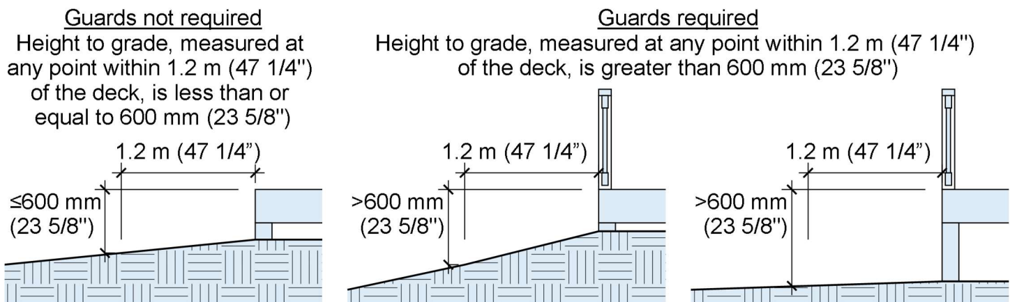
Figure 19 – Locations Where Guards Are Required
