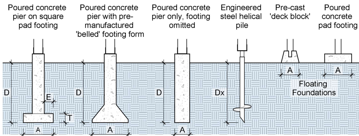
Figure 3 – Examples of Typical Foundation and Footing Types
