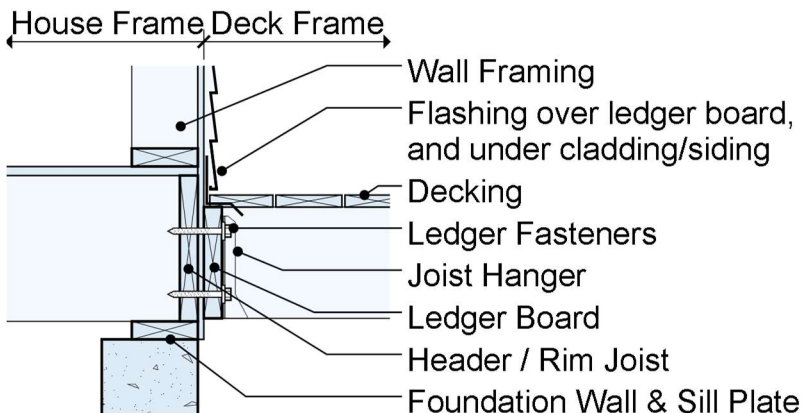
Figure 12 – Ledger Board Cross-section
