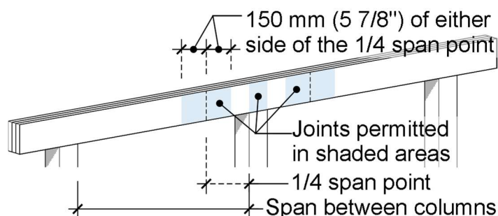
Figure 8 – Joints in 3-ply Built-up Beams
