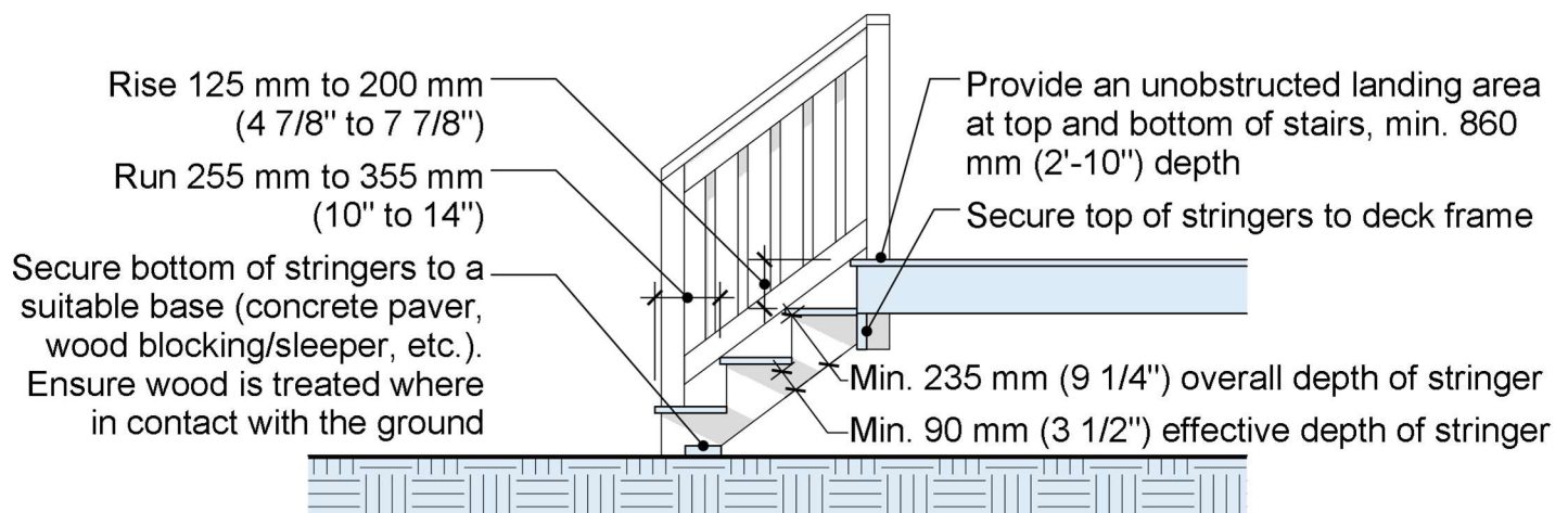
Figure 17 – Typical Stair Dimensions and Construction
