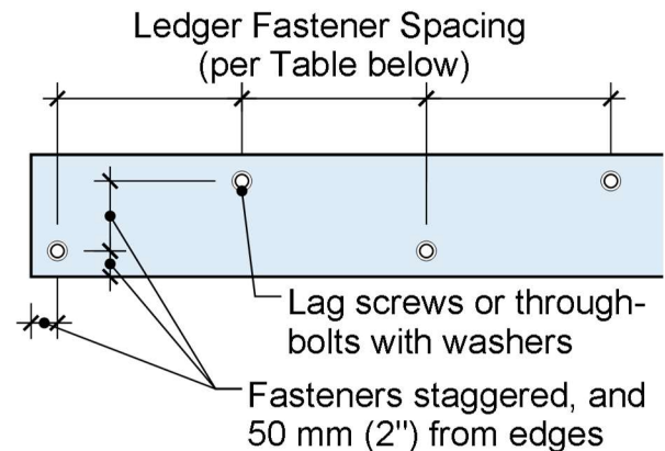
Figure 13 – Ledger Board Fastening Pattern
