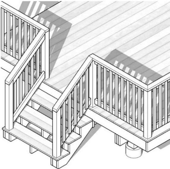
Figure 23 – SB-7 Cantilevered Picket System
