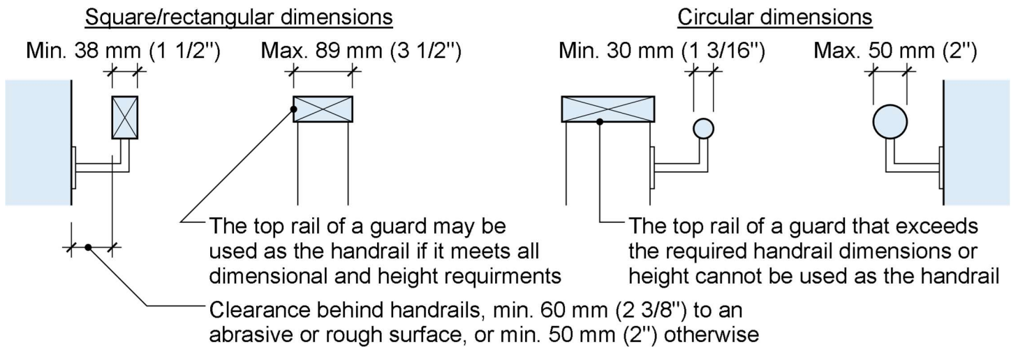
Figure 18 – Handrail Dimensions and Design Examples
