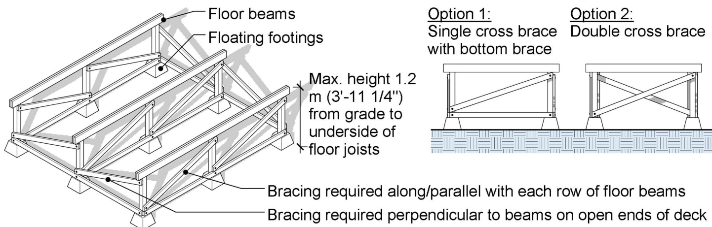
Figure 5 – Floating Deck Column Bracing Details
