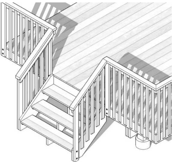
Figure 23 – SB-7 Cantilevered Picket System
