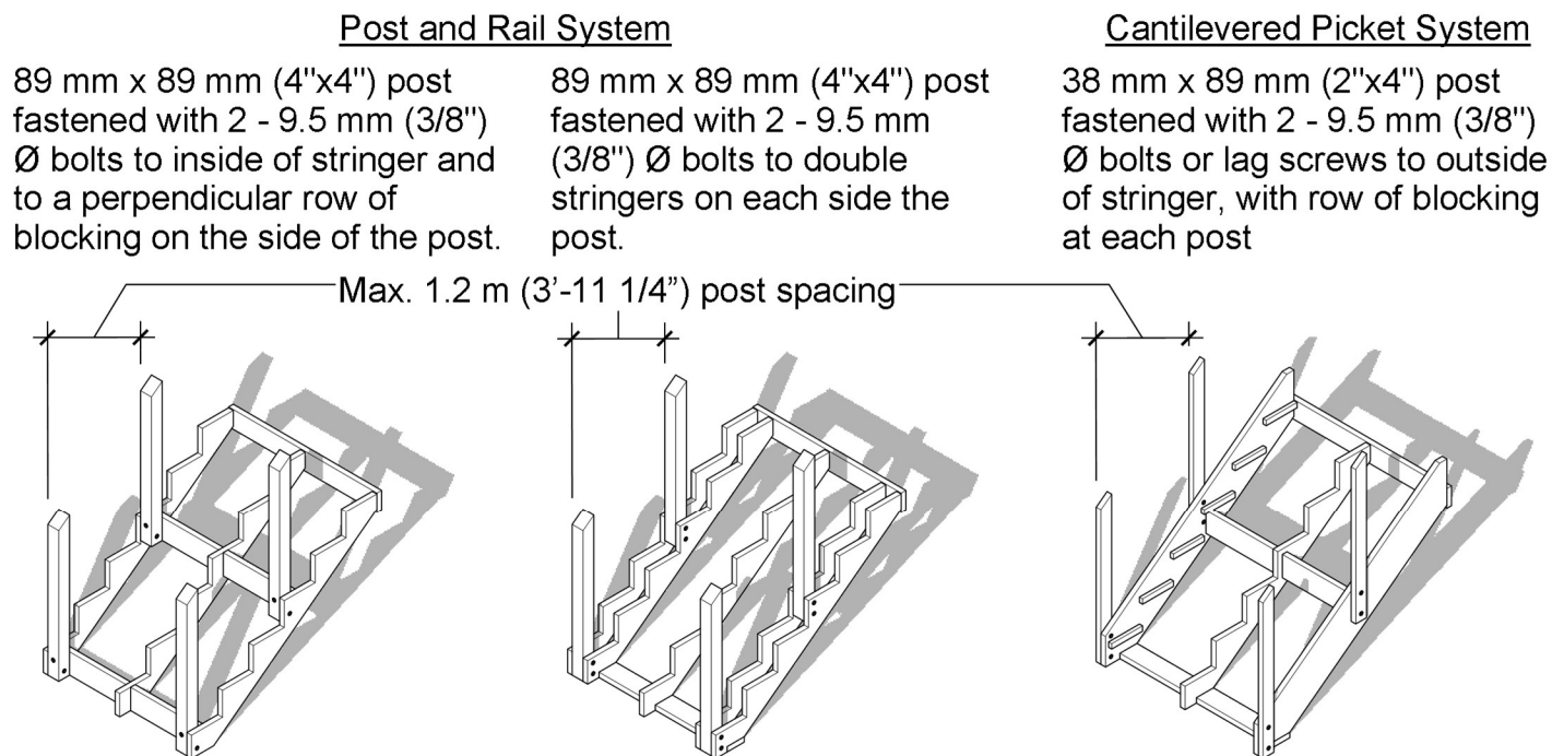
Figure 24 – Guard Post Fastening on Sides of Stairs
