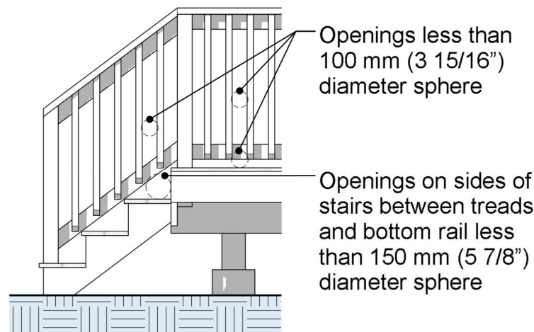
Figure 20 – Openings in Guards
