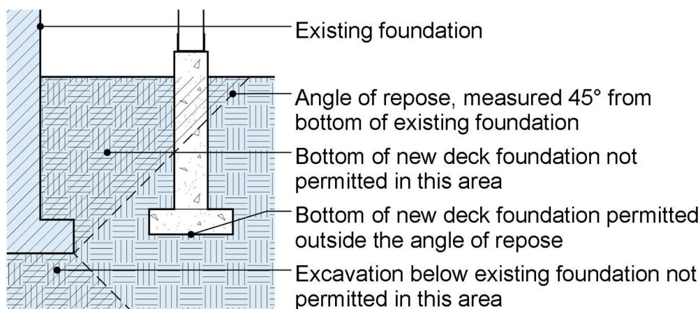
Figure 1 – Angle of Repose for Below Grade Footings
