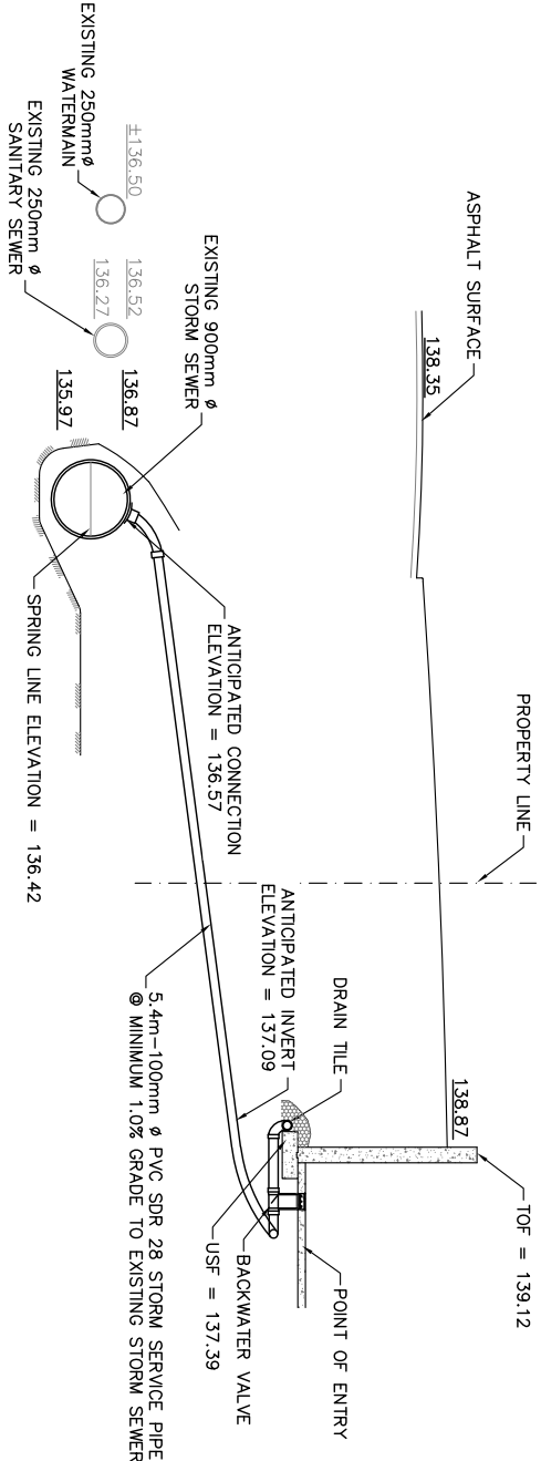
STORM CONNECTION DETAIL (NOT TO SCALE)
